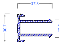
Hurricane Bar 3 Base PAM 127
