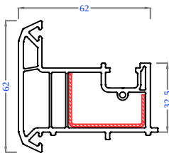
Movable Mullion PC62-UT-03
