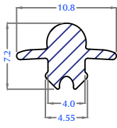
Sl.Track Rail PAM 101 (R07)
