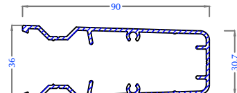
Hurricane Bar 3 cover PAM 128
