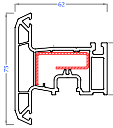
Window Sash - Outward Open PC62-US-01
