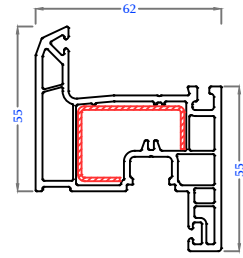
Window Sash - Inward Open - Tilt & Turn PC62-US-02
